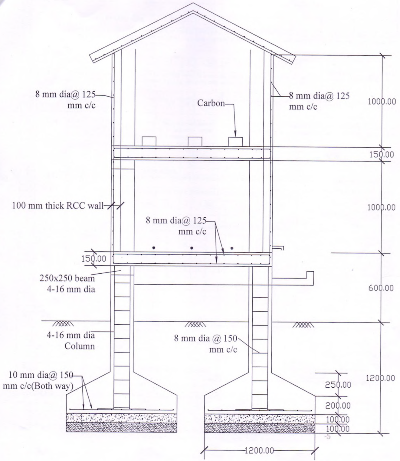
CROSS SECTION
